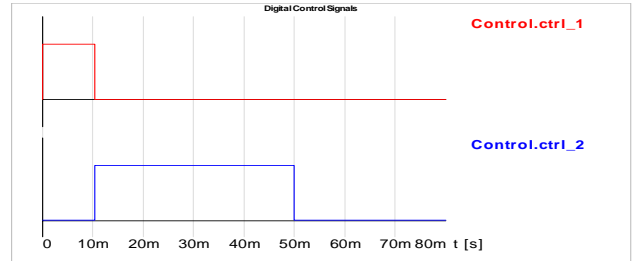
Figure 6: Control Signal Characteristics
