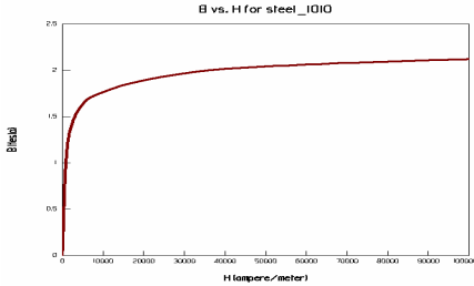
Figure 2: Non-linear Permeability Curve
