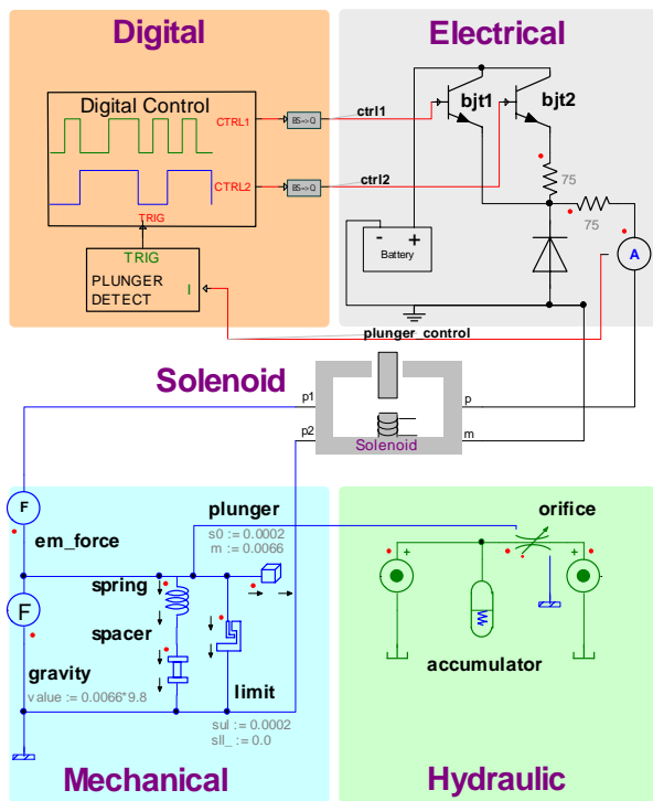
Figure 1: Linear Actuation System
