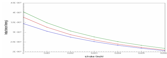
Figure 4: Per turn Inductance vs. Stroke for Various Coil Currents
