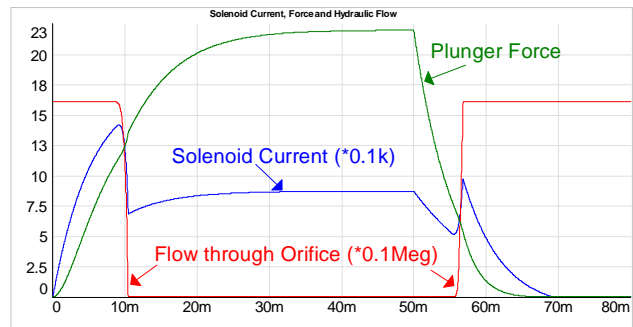
Figure 7: Solenoid Current, Force, and Hydraulic Flow
