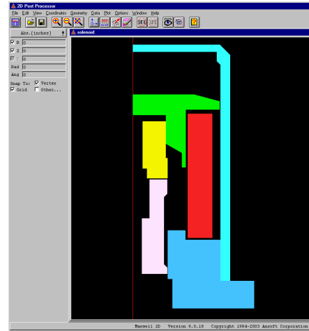
Figure 3: Cross section of the Solenoid
