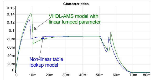
Figure 8: Comparison of Solenoid Current Characteristics
