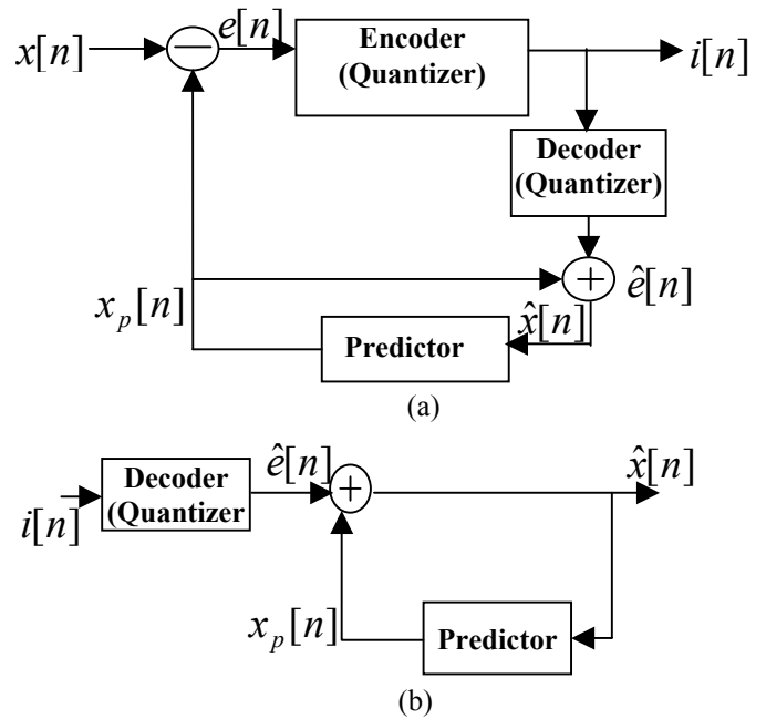
Figure .5. Differential Pulse coding (DPCM)
