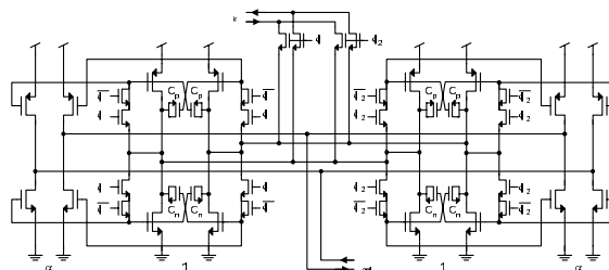
Figure 11: Transistor Level implementation of two-phase sampled filter
