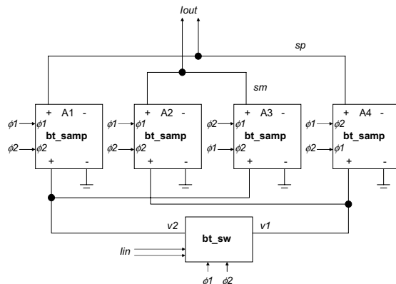
Figure 10: Block Structure of the proposed behavioural model
