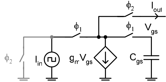
Figure 3. SI memory cell circuit model
