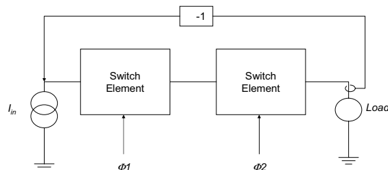
Figure 7: Basic Integrator Model
